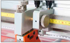
Fine position regulator for lengthwise cutters (optional)
